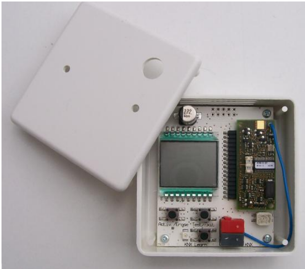
Figure 1: KNX ENO 620 with the top open
