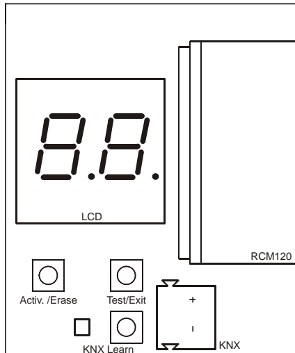
Figure 4: Device with the top open
