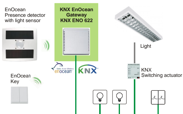
Figure 6: Application example: light controller
