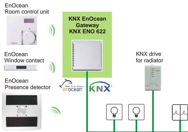
Figure 5: Application example: heating controller
